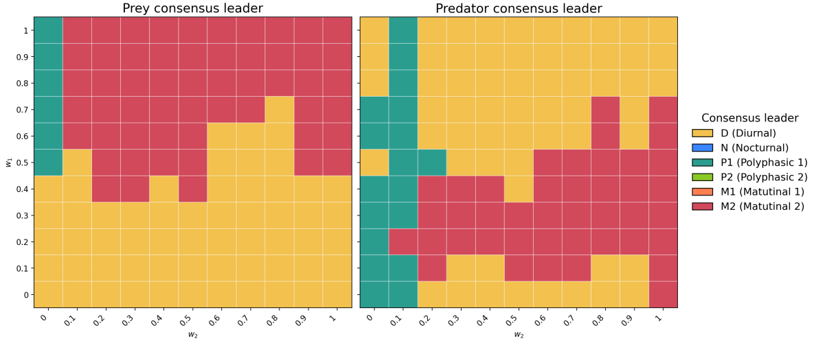
Figure 7: Consensus leading component of the mixed Nash equilibrium as a function of the prey sight weight w_1 and predator sight weight w_2 . Each cell corresponds to one weight pair and is labeled by the strategy with the largest probability in the unique mixed Nash equilibrium. The left panel shows the prey leader and the right panel shows the predator leader.
