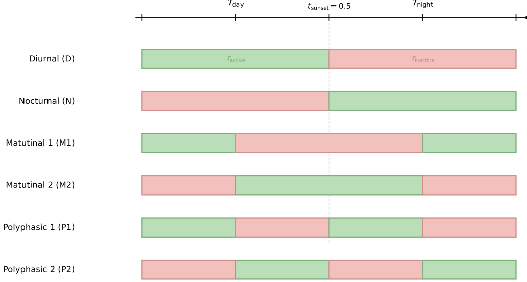
Figure 2: Standardized circadian activity schedules used in the simulations for a unit daily period with t_{\text{sunrise}} = 0 and t_{\text{sunset}} = 0.5 . The active sets are D = [0, 0.5) , N = [0.5, 1) , M_1 = [0, 0.25) \cup [0.75, 1) , M_2 = [0.25, 0.75) , P_1 = [0, 0.25) \cup [0.5, 0.75) , and P_2 = [0.25, 0.5) \cup [0.75, 1) .
