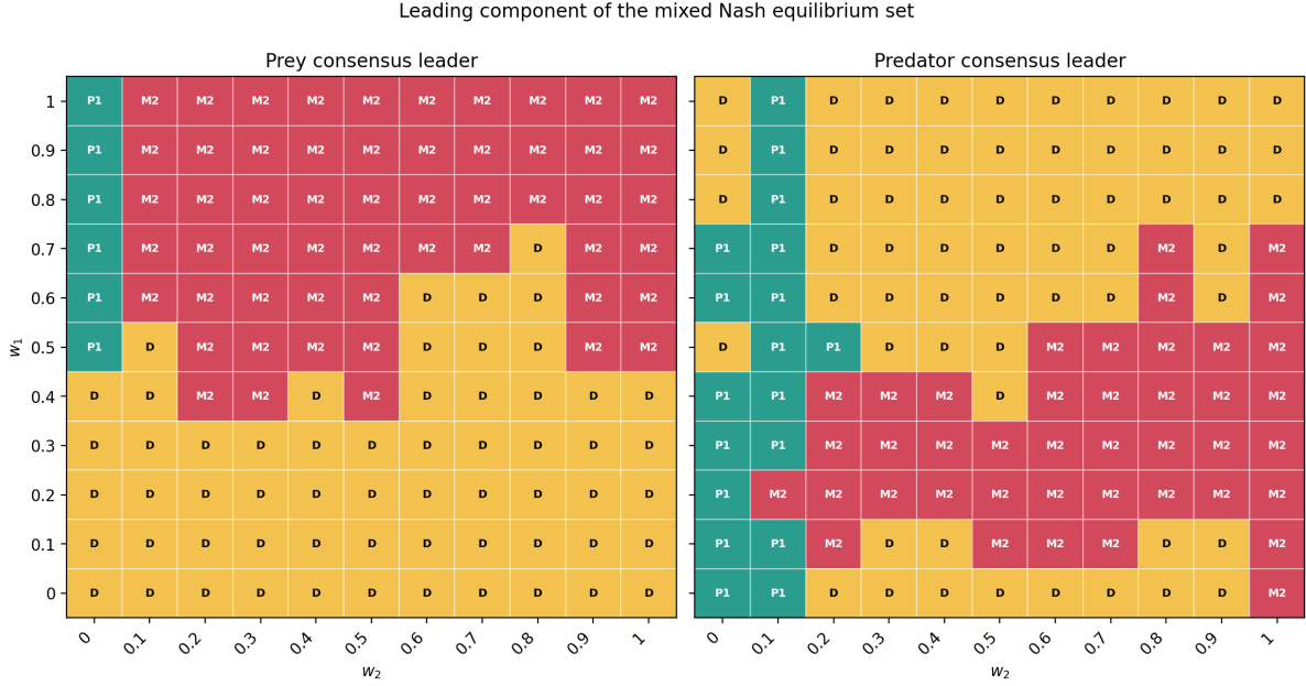
Figure 9: Consensus leading component of the mixed Nash equilibrium as a function of the prey sight weight w_1 and predator sight weight w_2 . Each cell corresponds to one weight pair and is labeled by the strategy with the largest probability in the unique mixed Nash equilibrium. The left panel shows the prey leader and the right panel shows the predator leader.
