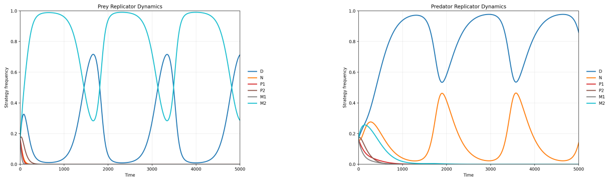
Figure 10: Representative asymmetric replicator dynamics for the balanced case (w_1, w_2) = (0.5, 0.5) , initialized from the uniform strategy distribution. Left: prey strategy frequencies. Right: predator strategy frequencies. The dominant strategies remain concentrated on the support highlighted by the mixed Nash equilibrium, but the trajectory exhibits persistent oscillations rather than monotone convergence to a fixed point.
