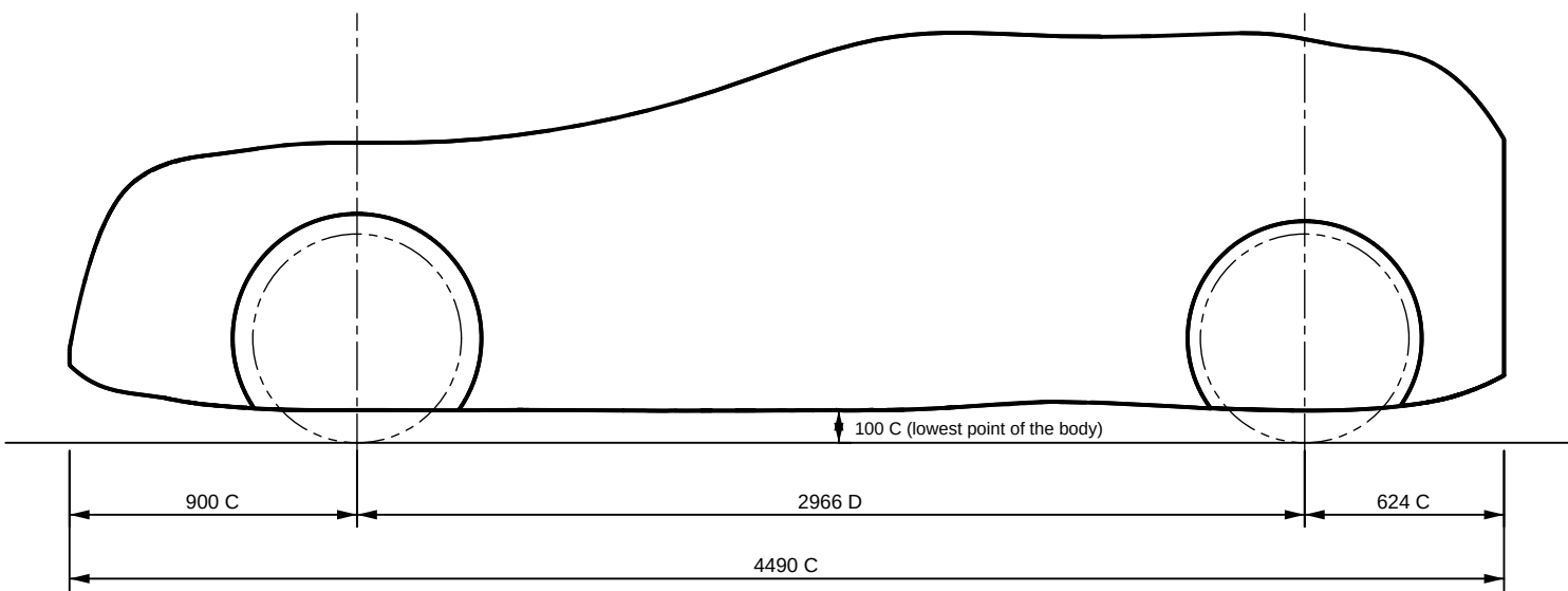
SIDE ELEVATION (left side)
