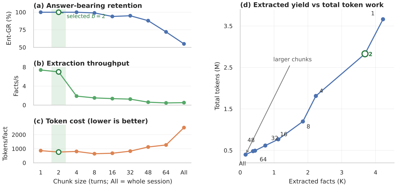
Figure 8: Chunk-size trade-off on the assembled-long-session diagnostic. (a)–(c) report retention, throughput, and per-fact token cost; (d), whose point labels denote chunk size, relates extracted-fact yield to total token work. Coarse chunks lower aggregate work partly by omitting facts rather than preserving quality at lower cost.
