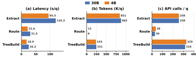
Figure 7: Per-question MemForest write-path breakdown under the 30B and 4B build backbones. Extraction dominates time and token use; parallel tree summaries account for many calls but a smaller wall-clock share.
