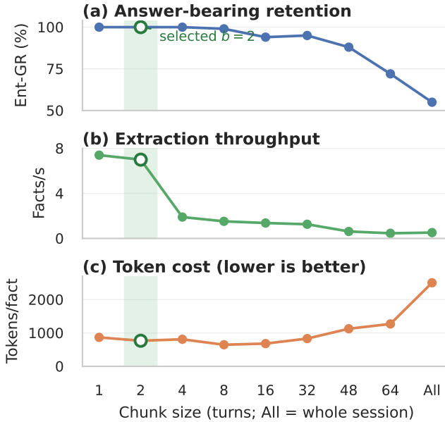
Figure 7: Chunk-size operating points on the assembled-long-session diagnostic. Ent-GR is the fraction of gold-range extractions retaining the answer-bearing span.
