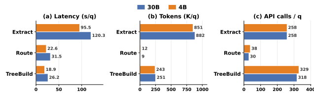
Figure 7: Per-question write-path breakdown of MemForest under the 30B and 4B build backbones. Extraction dominates both wall-clock time and token usage, whereas tree building contributes the most LLM calls but only a modest fraction of total time.
