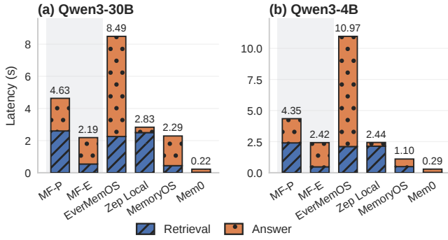
Figure 5: Retrieval and answer latency. MF-P and MF-E denote MemForest-Planner and MemForest-Embed.
