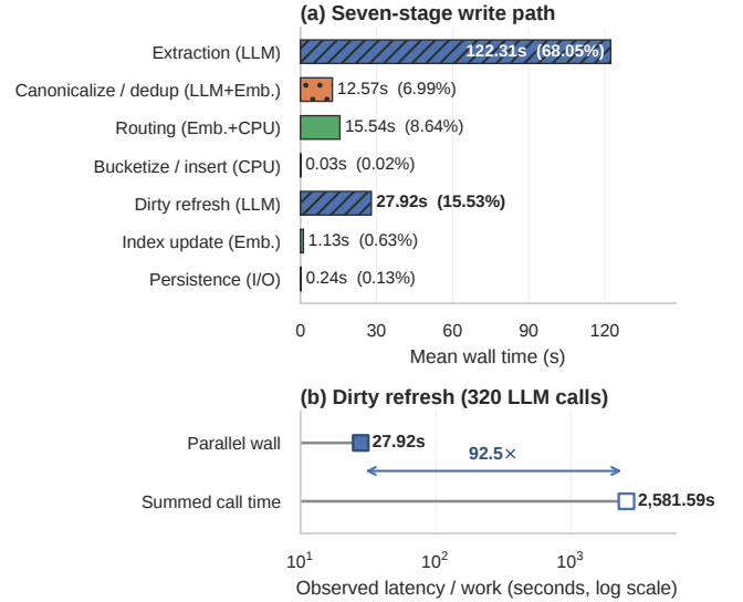
Figure 8: Detailed Qwen3-30B write-path profile, averaged over three representative LongMemEval streams (179.74 seconds total). (a) Each stage is labeled by its dominant workload. (b) The 320 dirty-refresh LLM calls sum to 2,581.59 call-seconds but complete in 27.92 seconds wall time; summed call time is observed work, not a timed serial implementation.
