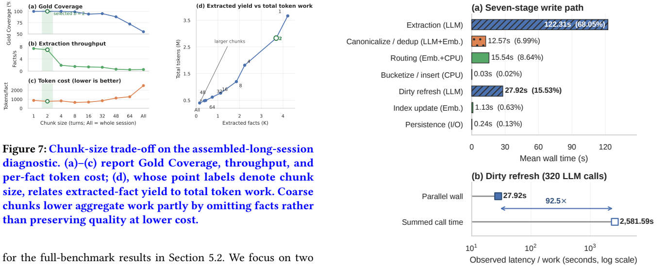
Figure 8: Detailed Qwen3-30B write-path profile, averaged over three representative LongMemEval streams (179.74 seconds total). (a) Each stage is labeled by its dominant workload. (b) The 320 dirty-refresh LLM calls sum to 2,581.59 call-seconds but complete in 27.92 seconds wall time; summed call time is observed work, not a timed serial implementation.
