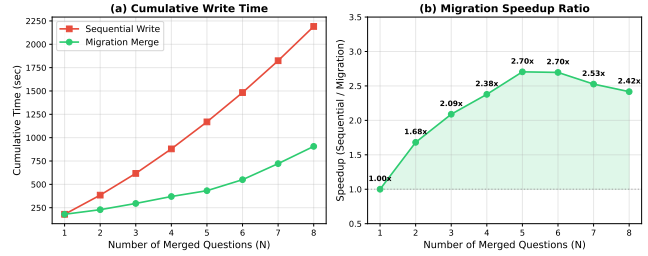
Figure 5: Migration efficiency on progressively merged LongMemEval instances. Left: cumulative maintenance time under sequential write and migration merge. Right: speedup of migration relative to sequential write.
