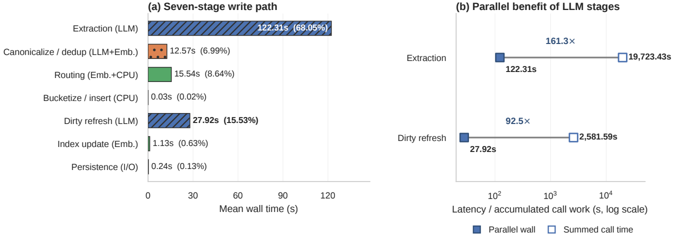
Figure 8: Detailed Qwen3-30B write-path profile, averaged over three representative LongMemEval streams (179.74 seconds total). (a) Each stage is labeled by its dominant workload. (b) Extraction and dirty refresh compare parallel wall time with summed observed LLM-call time; the latter is accumulated work, not a timed serial implementation.
