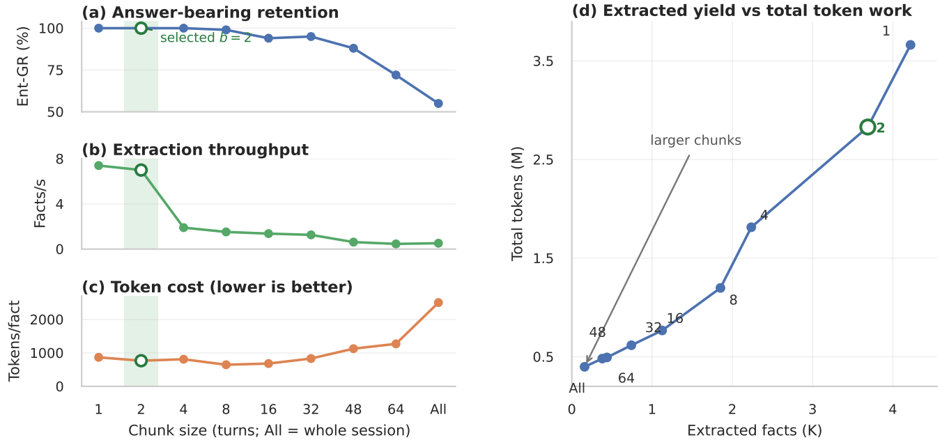
Figure 7: Chunk-size trade-off on the assembled-long-session diagnostic. (a)–(c) report retention, throughput, and per-fact token cost; (d), whose point labels denote chunk size, relates extracted-fact yield to total token work. Coarse chunks lower aggregate work partly by omitting facts rather than preserving quality at lower cost.
