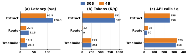
Figure 8: Per-question MemForest write-path breakdown under the 30B and 4B build backbones. Extraction dominates time and token use; parallel tree summaries account for many calls but a smaller wall-clock share.
