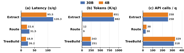
Figure 7: Per-question write-path breakdown of MemForest under the 30B and 4B build backbones. Extraction dominates both wall-clock time and token usage, whereas tree building contributes the most LLM calls but only a modest fraction of total time.
