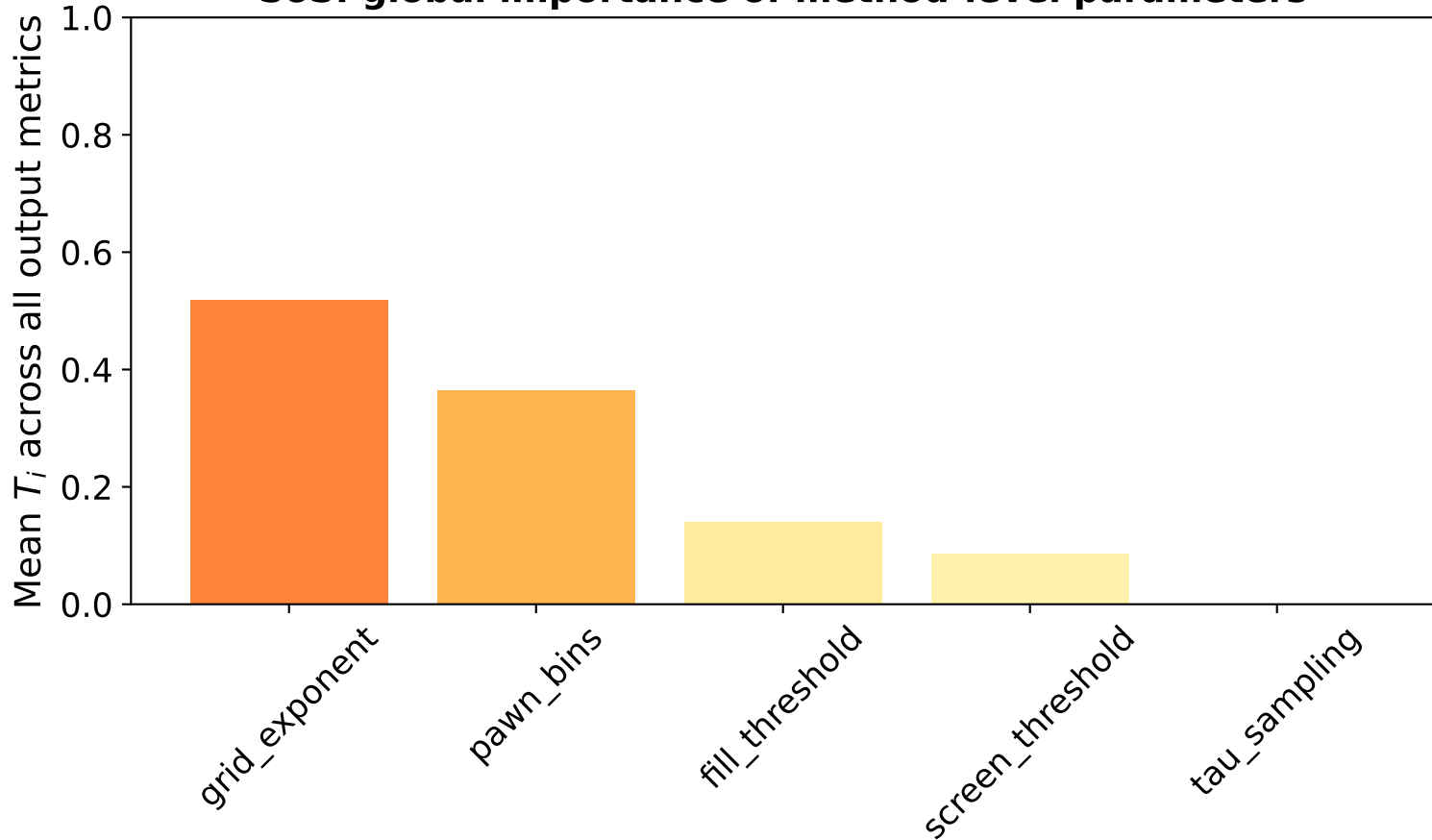
SoS: global importance of method-level parameters
