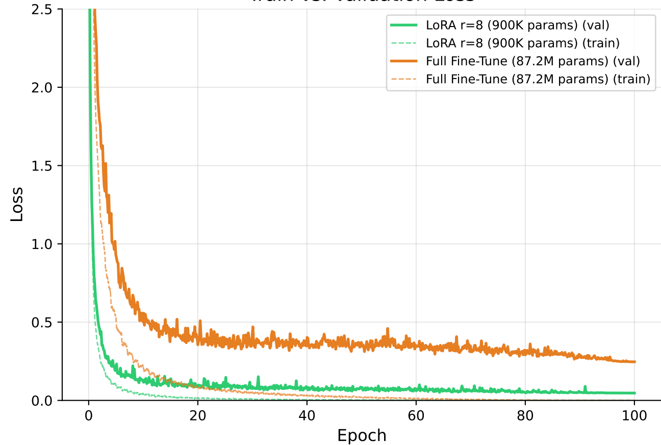
Train vs. Validation Loss
