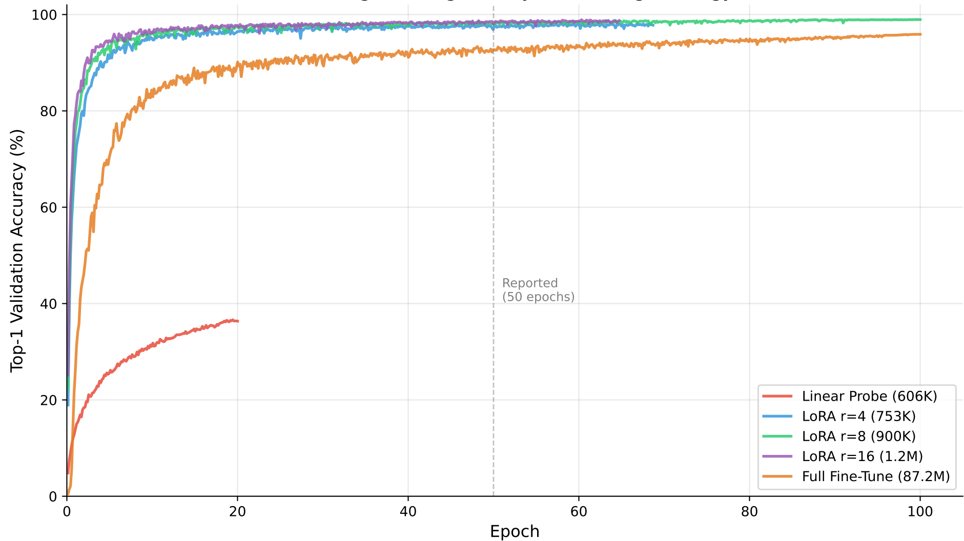
Training Convergence by Fine-Tuning Strategy
