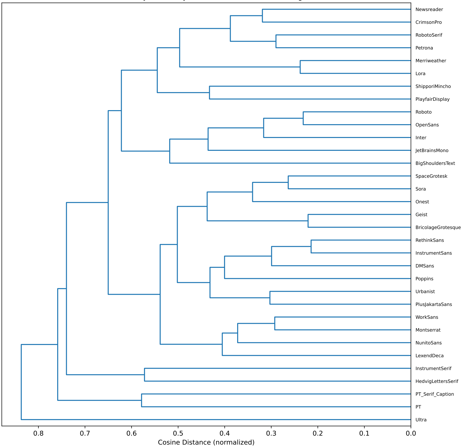
Font Family Similarity (UPGMA of [CLS] Embeddings)
