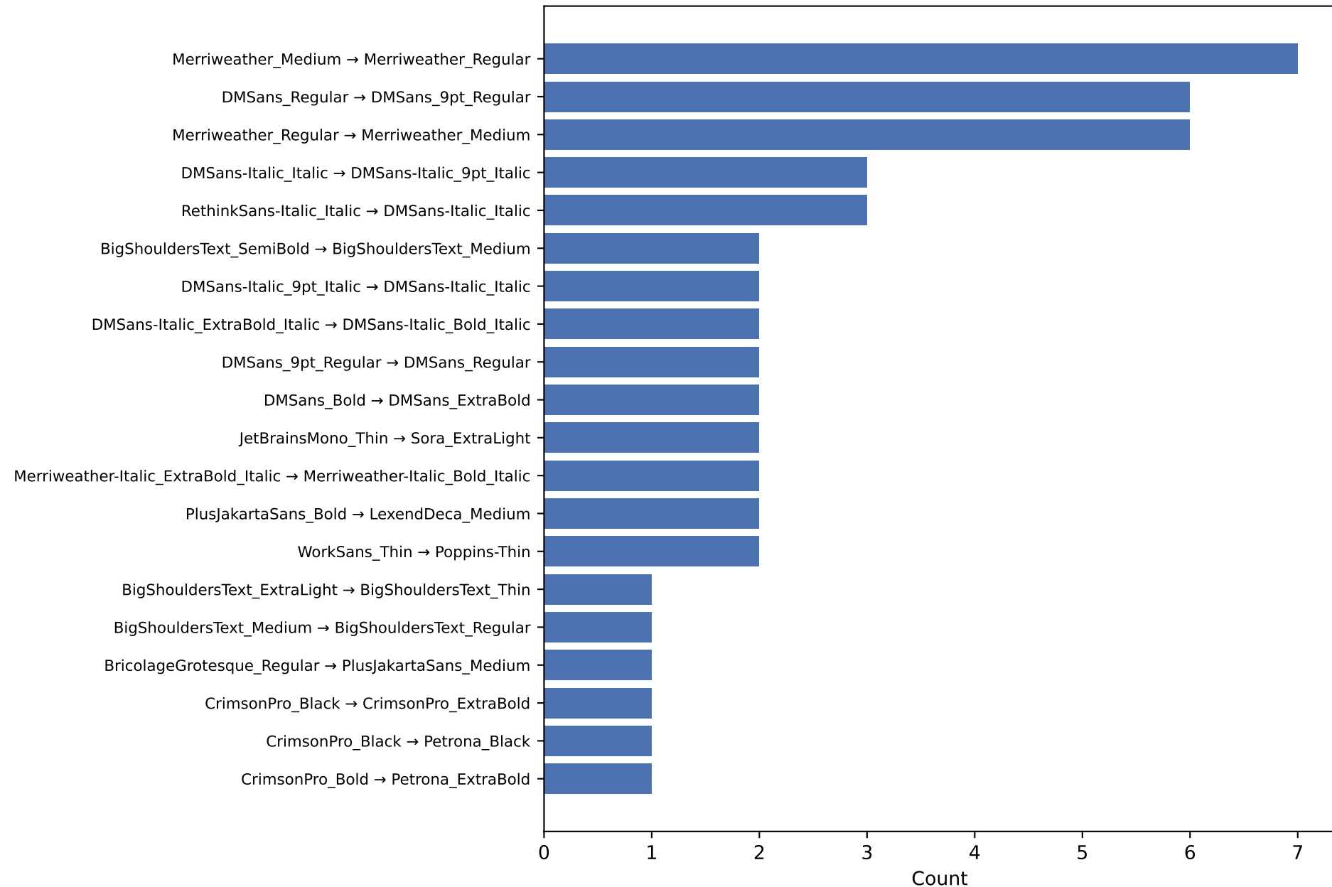
Top-20 Most Frequent Misclassifications
