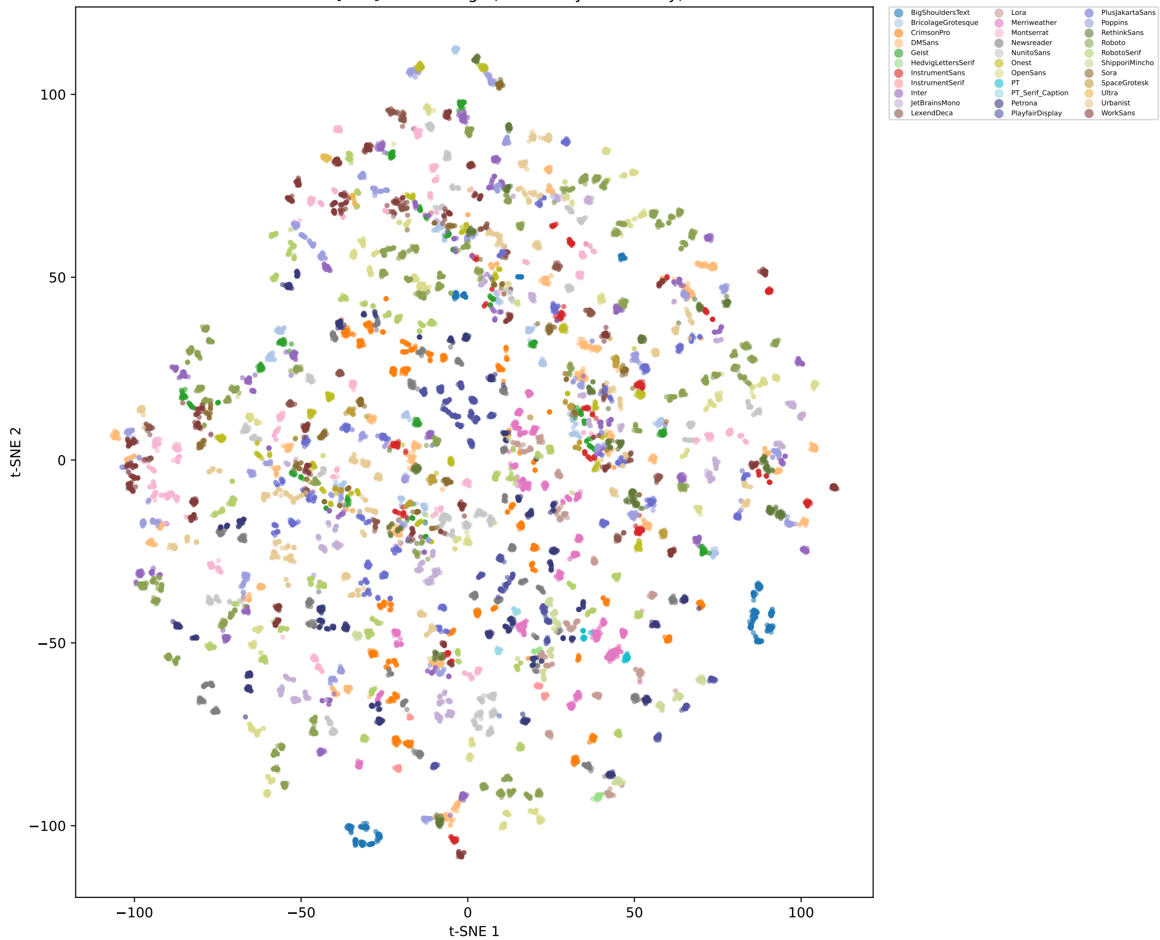
t-SNE of [CLS] Embeddings (colored by font family)
