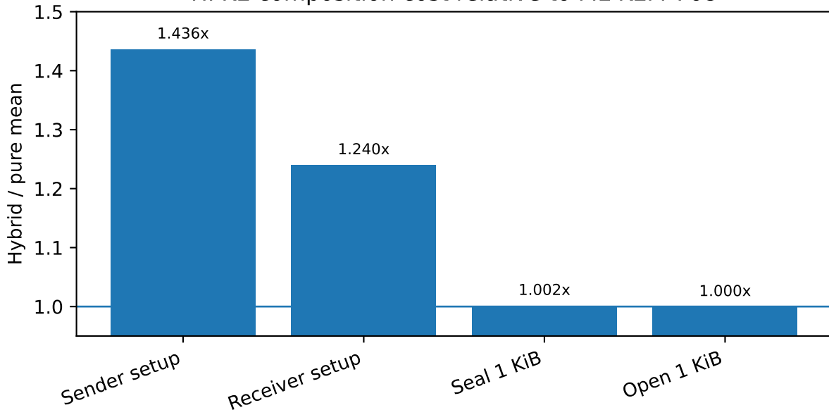
HPKE composition cost relative to ML-KEM-768
