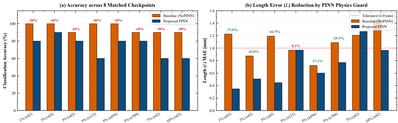
Figure 16: Head-to-Head Paired Checkpoint Comparison: PINN vs NoPINN Baseline
