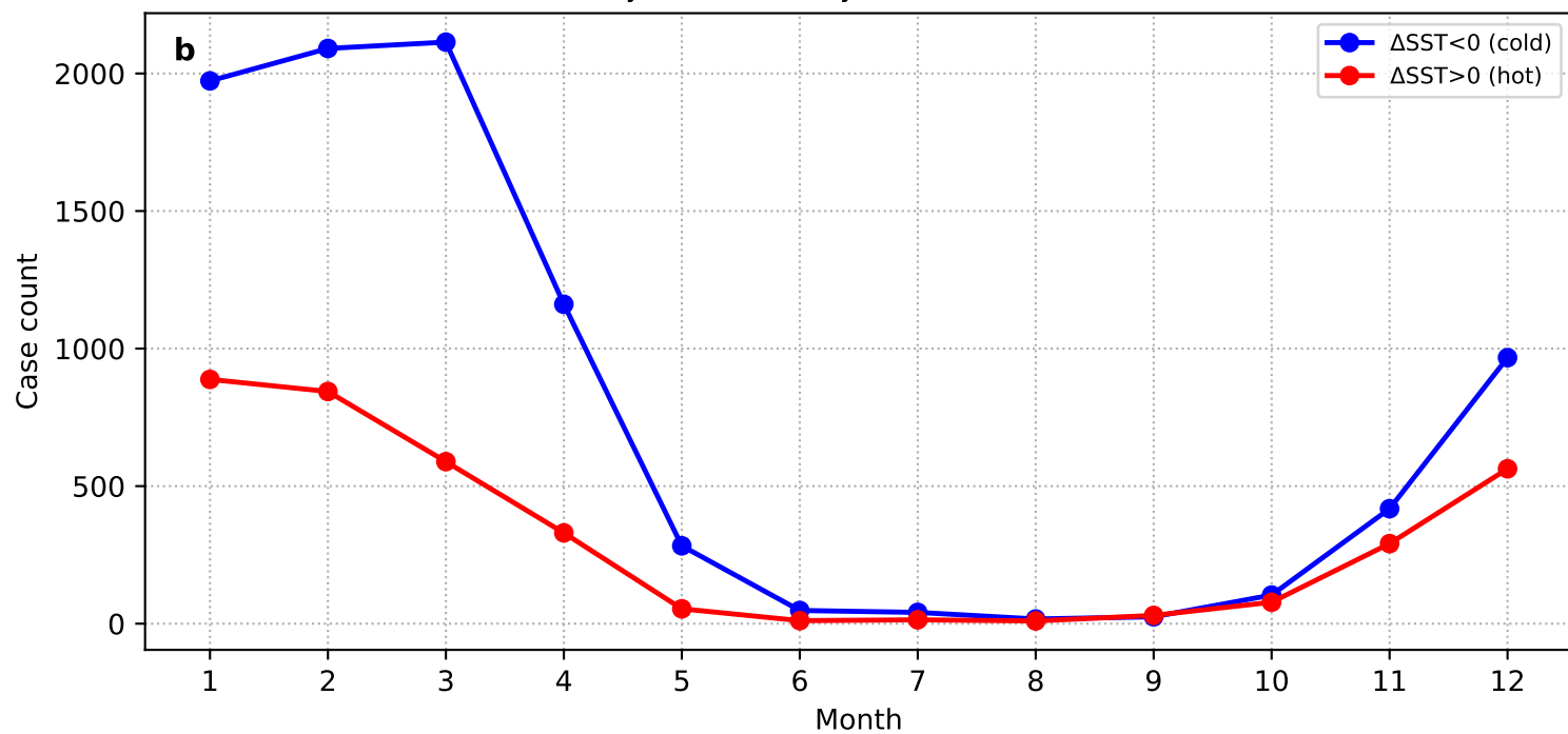
\Delta SST: Day 0 – mean(Day –10...–4) (SH + HYCOM)
