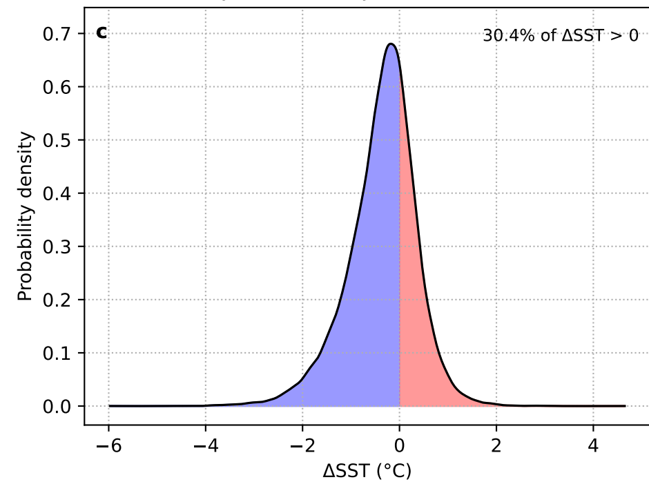
\Delta SST: Day 0 – mean(Day –10...–4) (GL + HYCOM)
