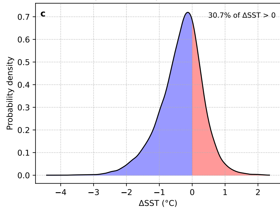
\Delta SST: Day 0 – mean(Day –10...–4) (SH + HYCOM)
