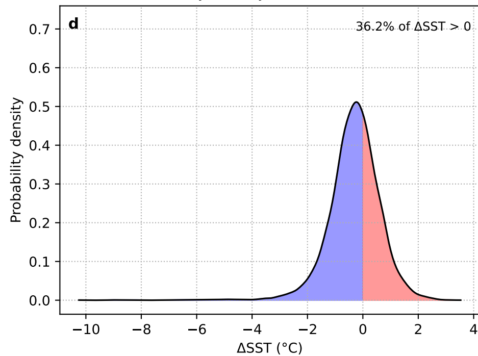
\Delta SST: Day 0 – Day –15 (SH + HYCOM)
