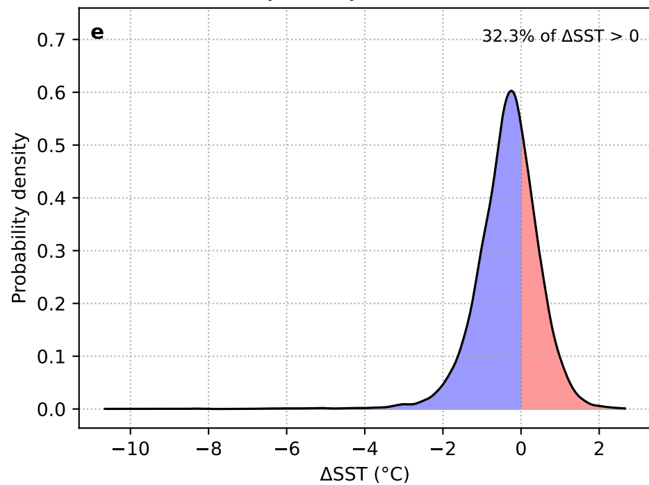
\Delta SST: Day 0 – Day –10 (SH + HYCOM)
