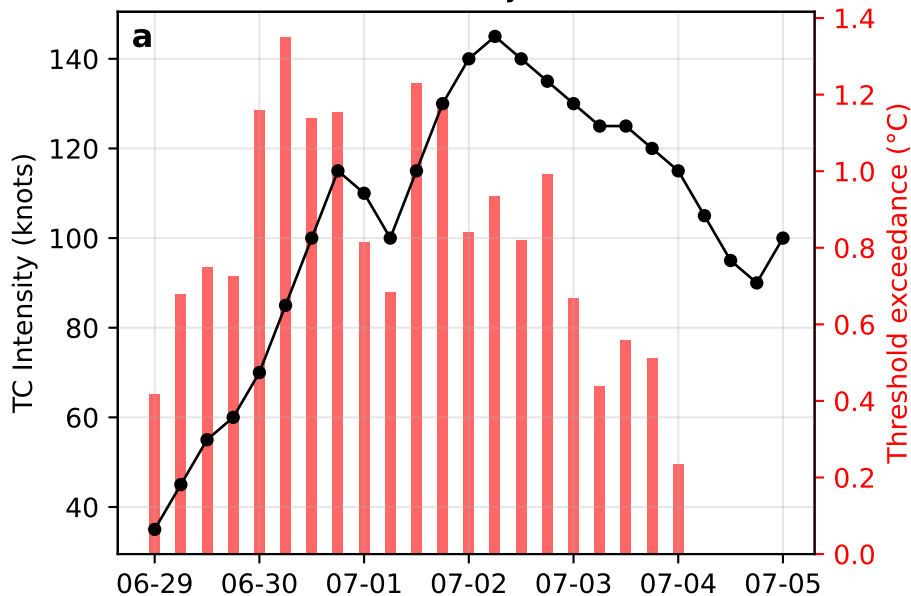
Hurricane Beryl (2024)
