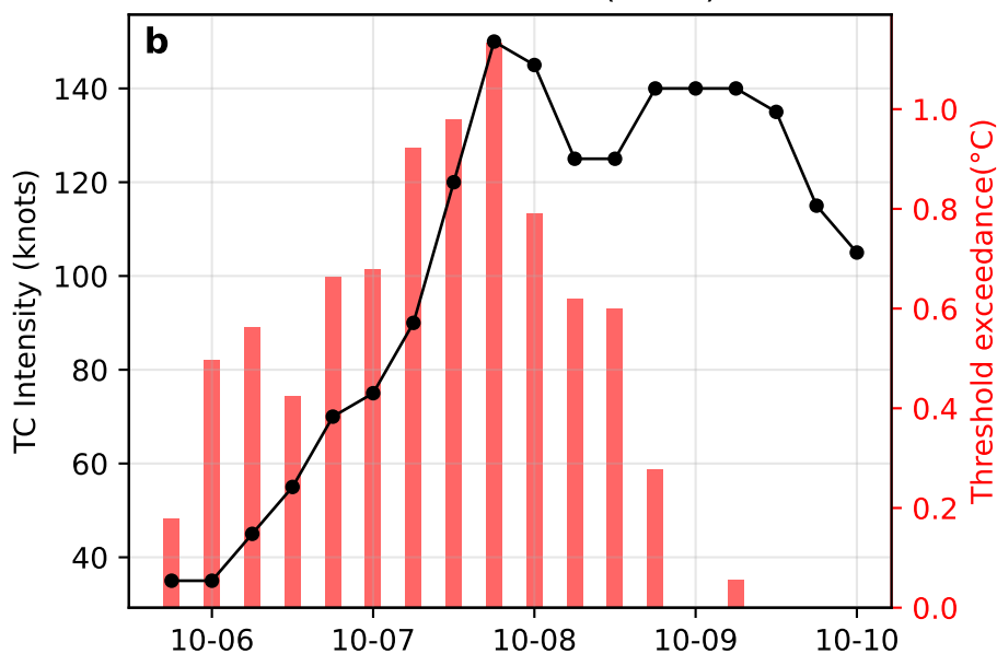
Hurricane Milton (2024)
