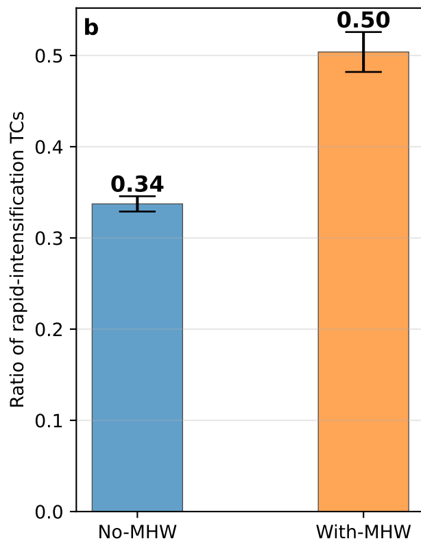
GL: MHW baseline 1992-2021
