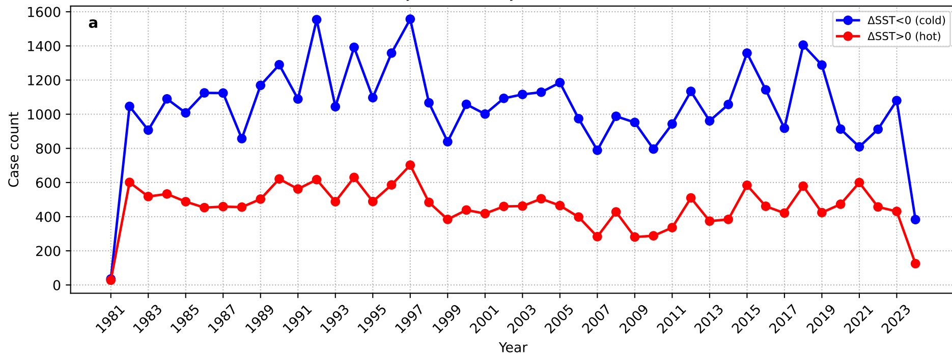
\Delta SST: Day 0 – mean(Day –10...–4) (GL + OISST)
