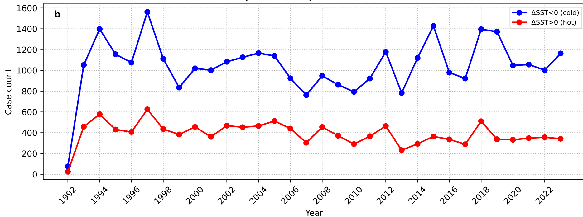
\Delta SST: Day 0 – mean(Day –10...–4) (GL + HYCOM)
