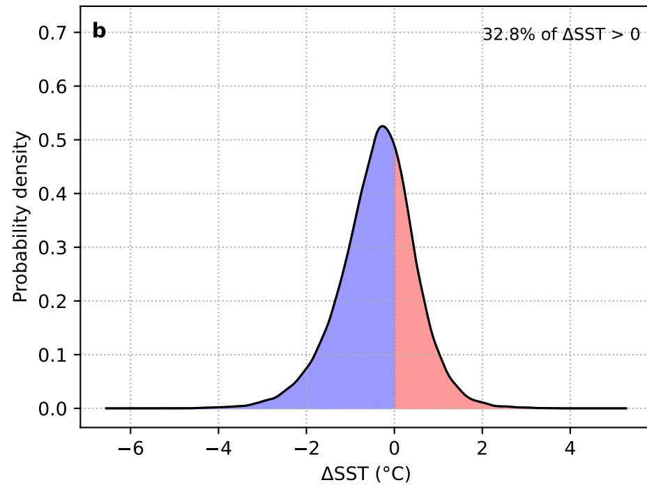
\Delta SST: Day 0 – Day –10 (GL + HYCOM)
