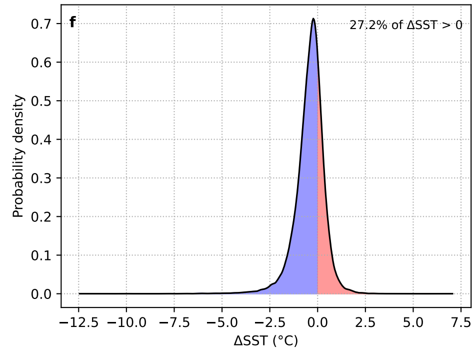
\Delta SST: Day 0 – mean(Day –10...–4) (GL + HYCOM)
