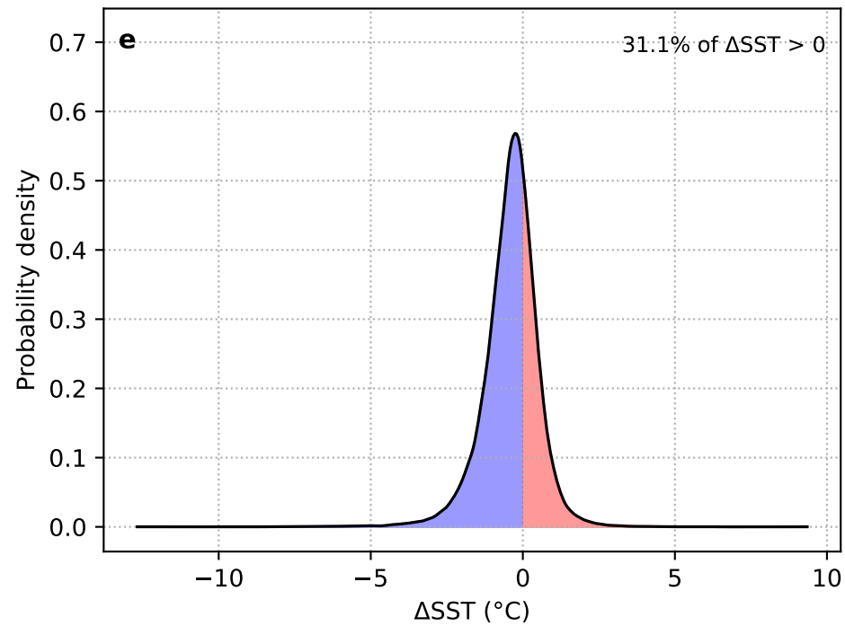
\Delta SST: Day 0 – Day –10 (GL + HYCOM)
