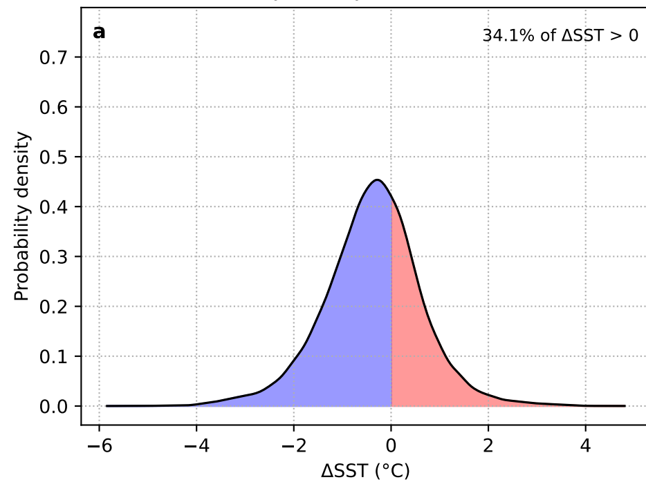
\Delta SST: Day 0 – Day –15 (WP + HYCOM)
