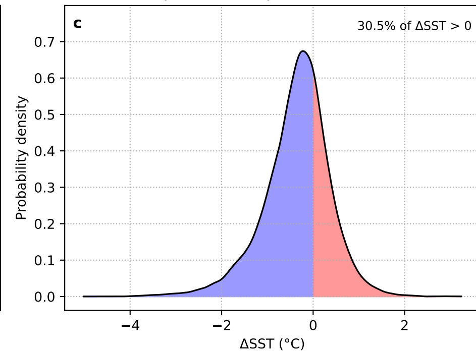
\Delta SST: Day 0 – mean(Day –10...–4) (WP + HYCOM)
