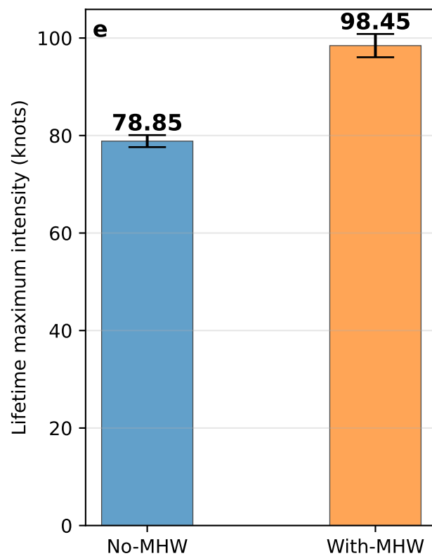
WP: MHW baseline 1982-2011
