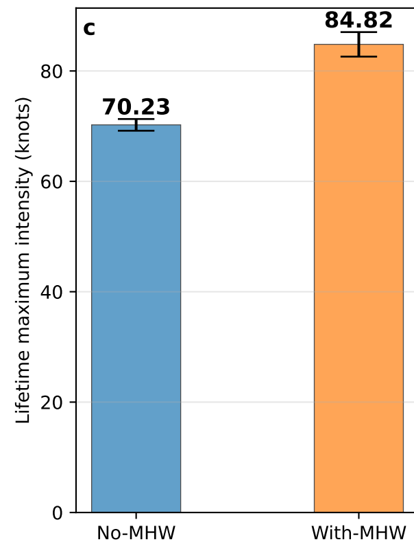
SH: MHW baseline 1982-2011
