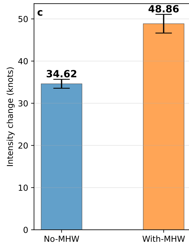
SH: MHW baseline 1982-2011
