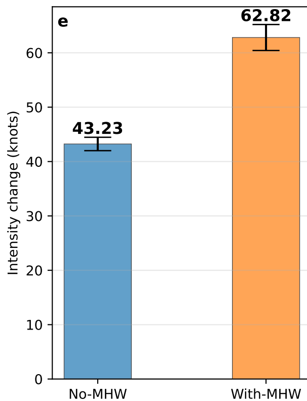
WP: MHW baseline 1982-2011
