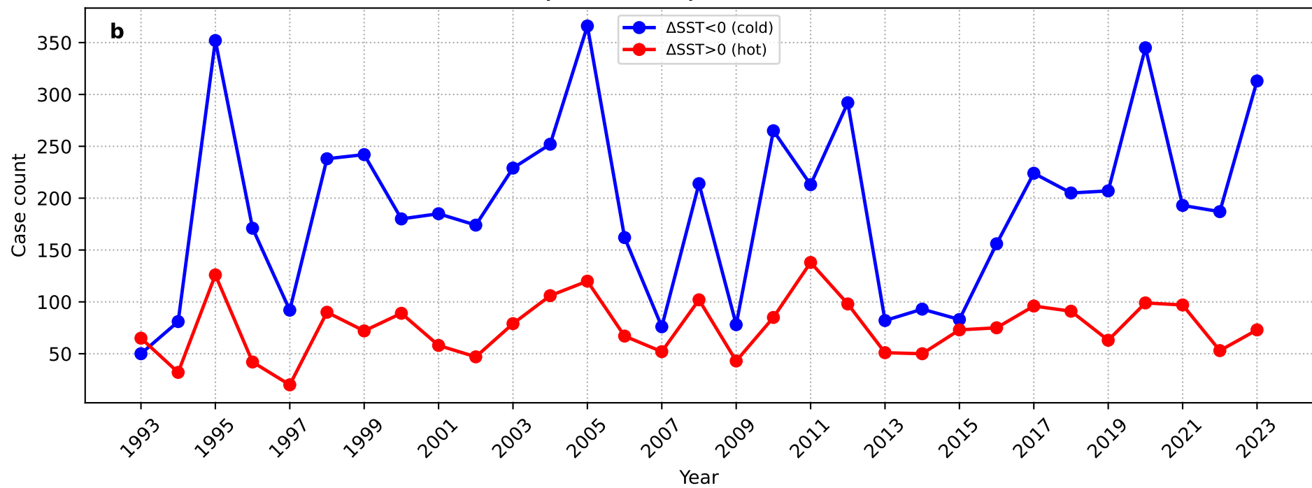
\Delta SST : Day 0 – mean(Day –10...–4) (AL + HYCOM)
