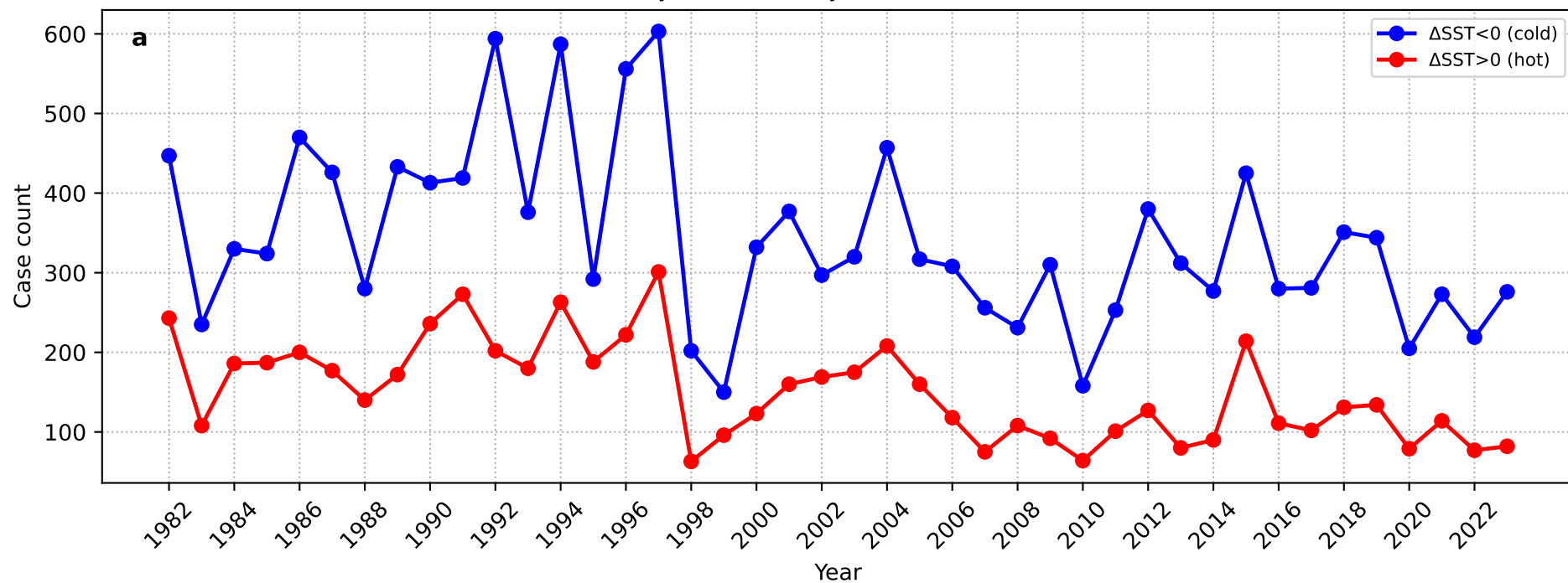
\Delta SST: Day 0 – mean(Day –10...–4) (WP + HYCOM)
