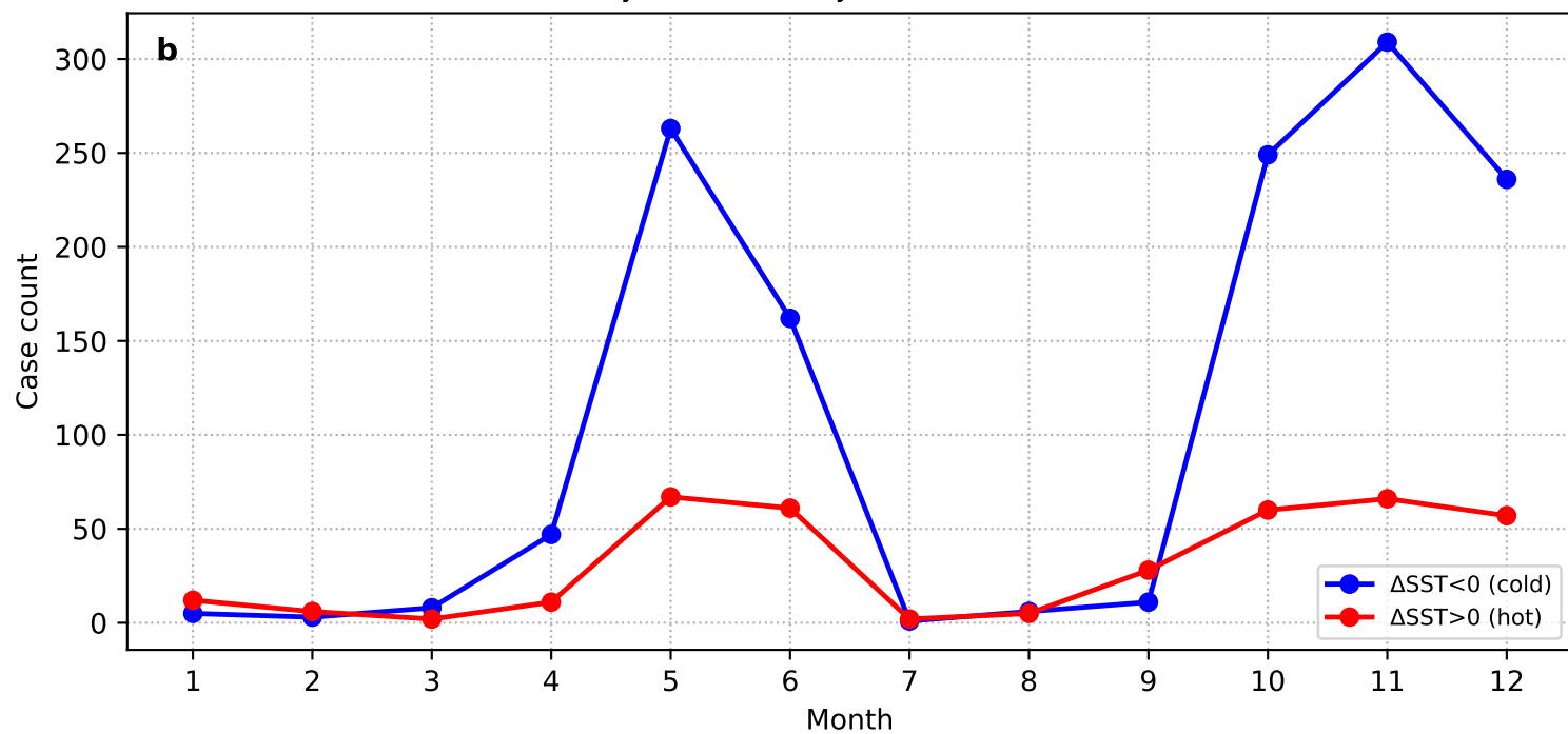
\Delta SST: Day 0 – mean(Day –10...–4) (IO + HYCOM)
