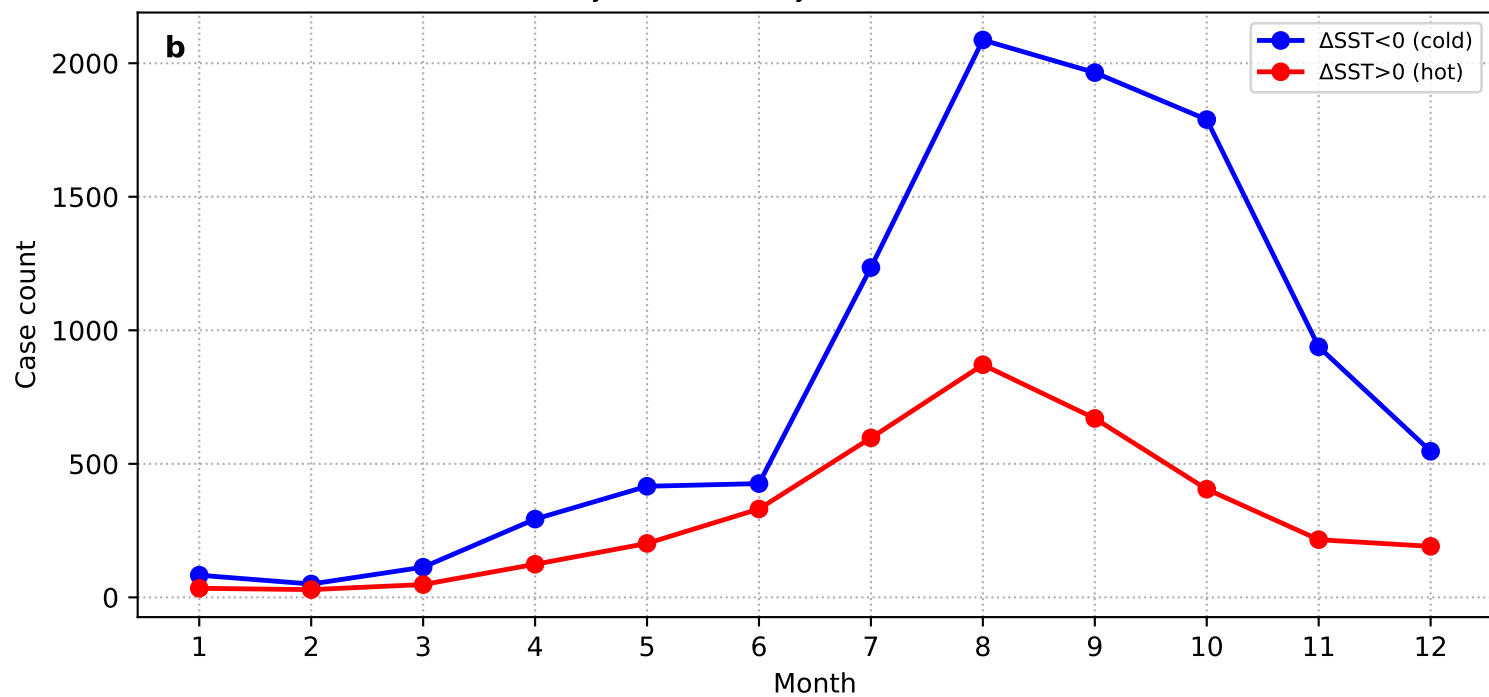
\Delta SST: Day 0 – mean(Day –10...–4) (WP + HYCOM)
