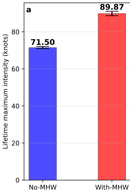
GL: MHW baseline 1982–2011
