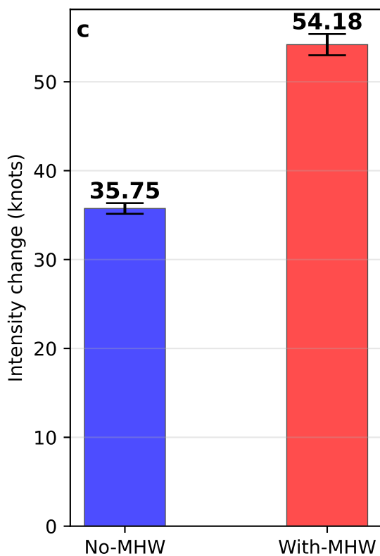
GL: MHW baseline 1982–2011
