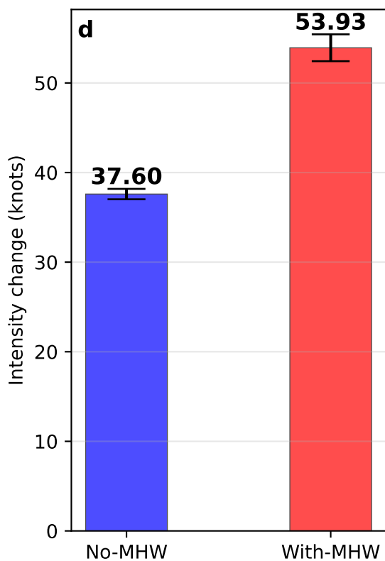
GL: MHW baseline 1992–2021
