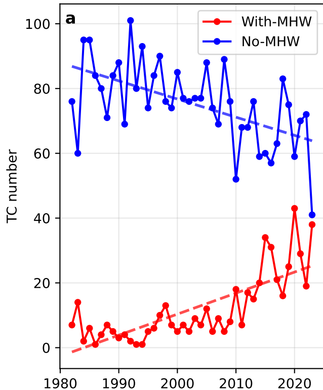
GL: MHW baseline 1992-2021
