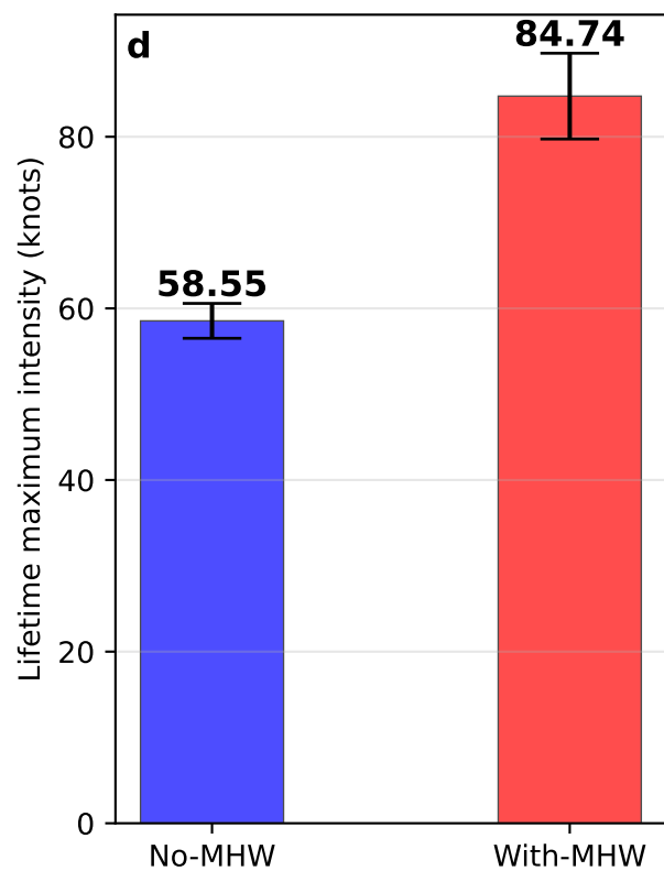
IO: MHW baseline 1992-2021
