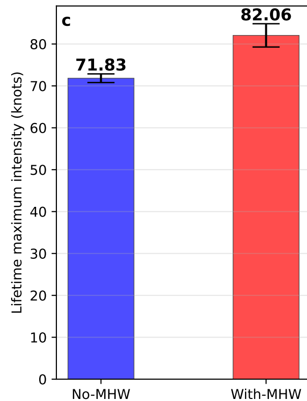
SH: MHW baseline 1992-2021
