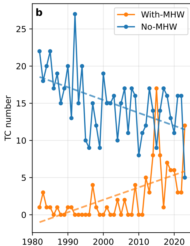
WP: MHW baseline 1992-2021
