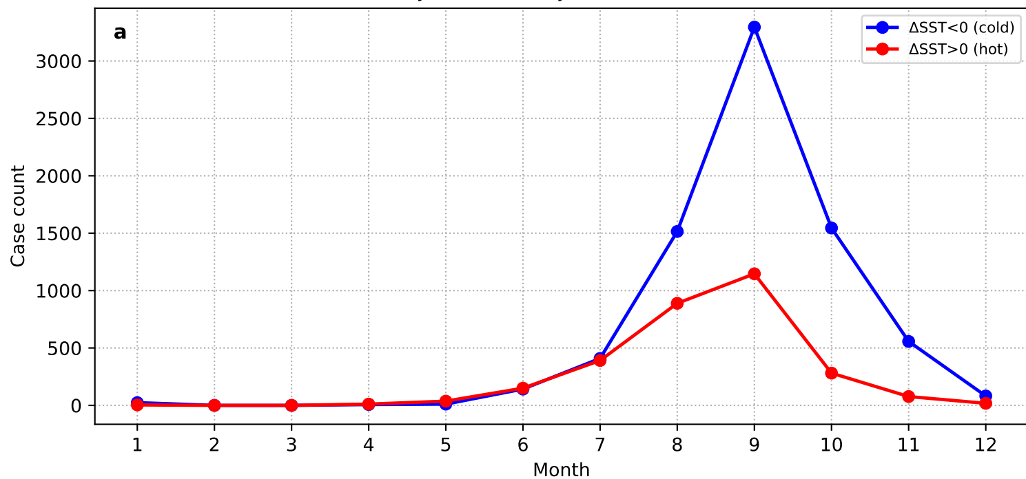
\Delta SST: Day 0 – mean(Day –10...–4) (AL + HYCOM)
