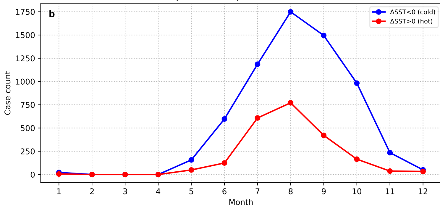
\Delta SST: Day 0 – mean(Day –10...–4) (EP + HYCOM)
