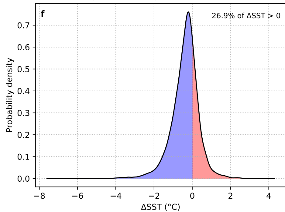
\Delta SST: Day 0 – mean(Day –10...–4) (WP + HYCOM)
