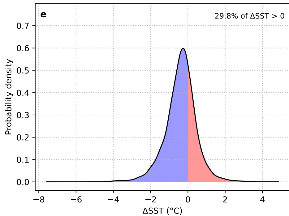
\Delta SST: Day 0 – Day –10 (WP + HYCOM)
