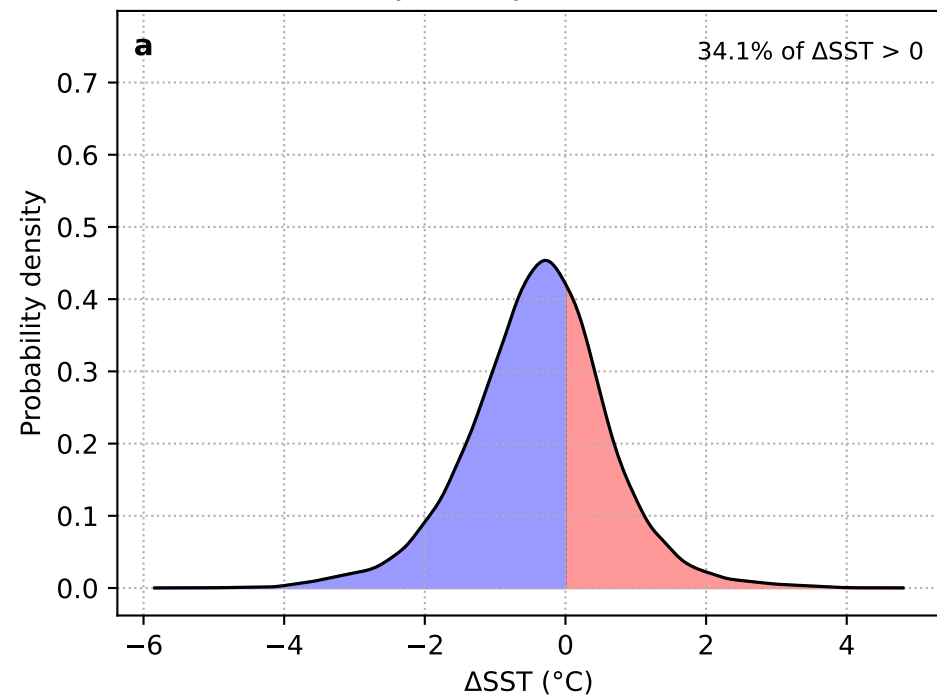
\Delta SST: Day 0 – Day –15 (WP + HYCOM)
