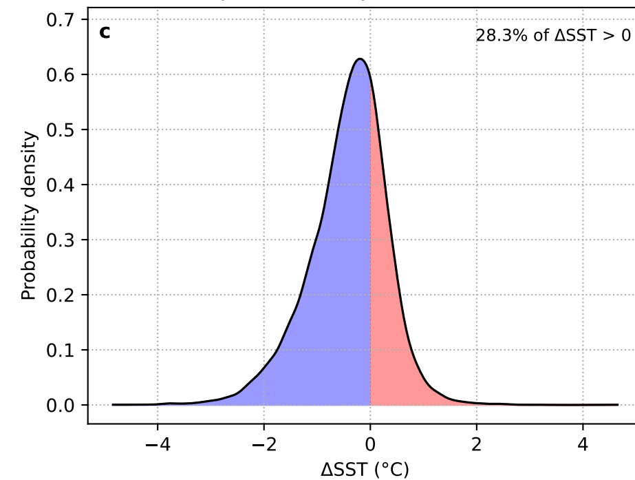
\Delta SST: Day 0 – mean(Day –10...–4) (AL + HYCOM)
