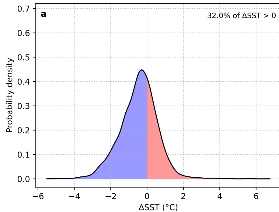
\Delta SST: Day 0 – Day –15 (AL + HYCOM)
