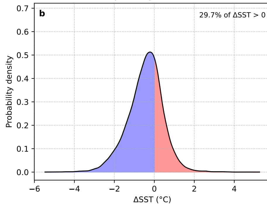
\Delta SST: Day 0 – Day –10 (AL + HYCOM)
