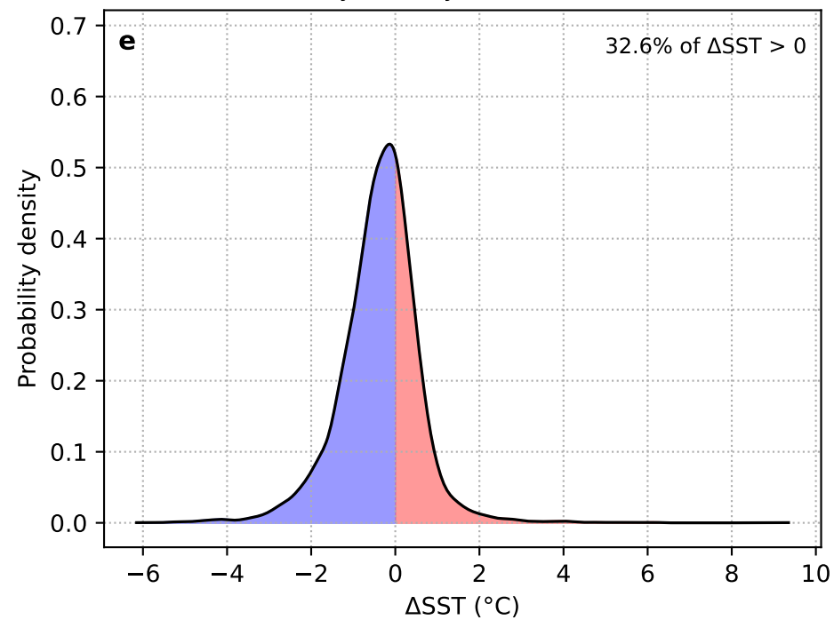
\Delta SST: Day 0 – Day –10 (AL + HYCOM)
