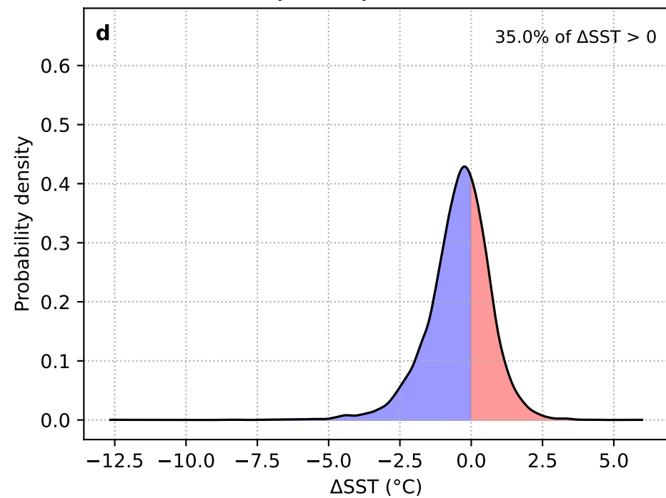
\Delta SST: Day 0 – Day –15 (EP + HYCOM)
