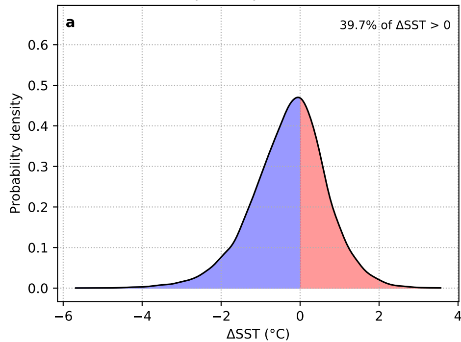
\Delta SST: Day 0 – Day –15 (EP + HYCOM)
