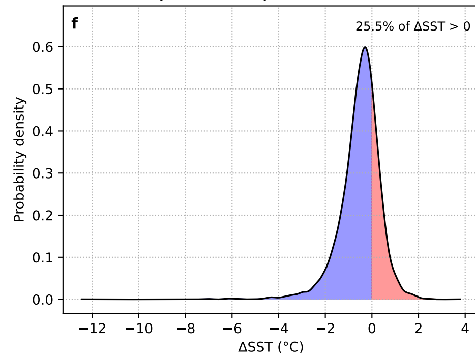
\Delta SST: Day 0 – mean(Day –10...–4) (EP + HYCOM)
