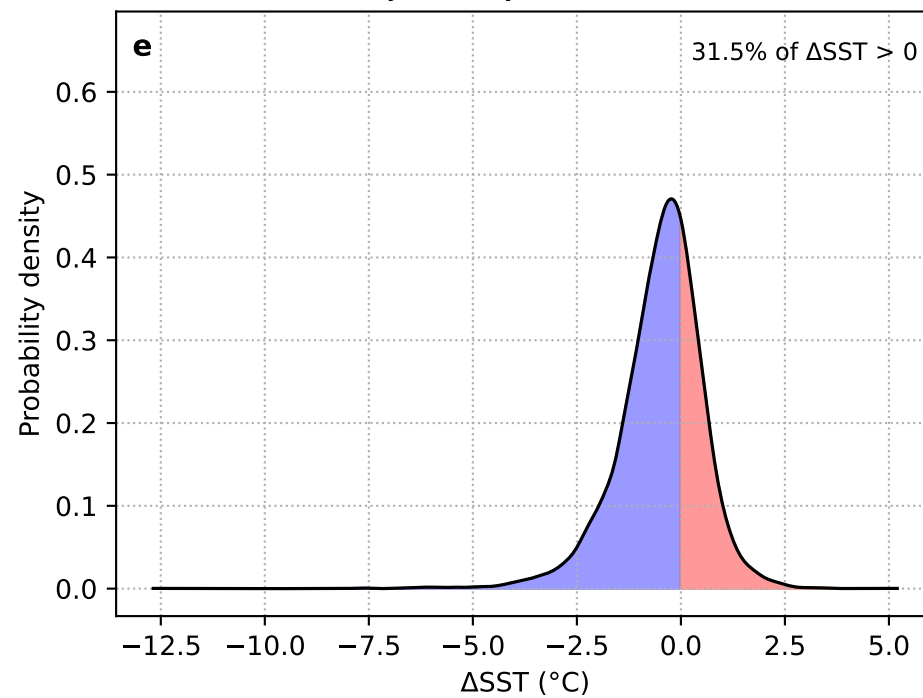
\Delta SST: Day 0 – Day –10 (EP + HYCOM)
