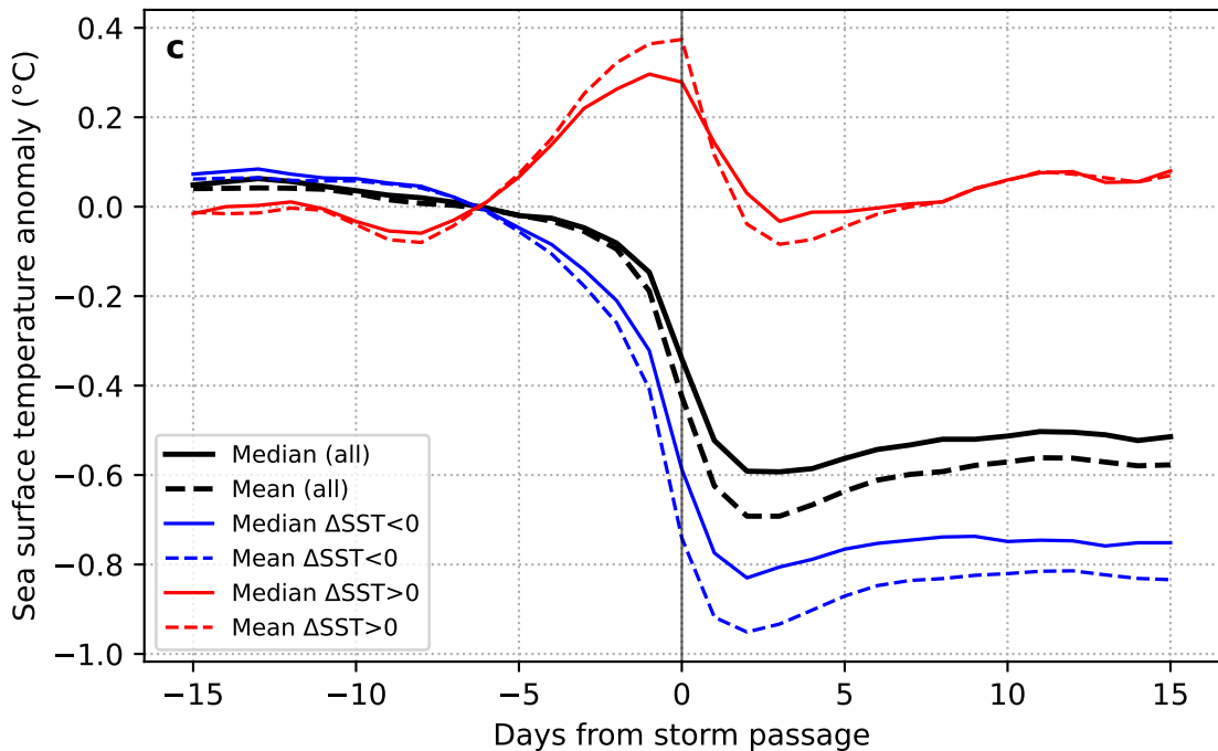
\Delta SST: Day 0 – mean(Day –10...–4)
