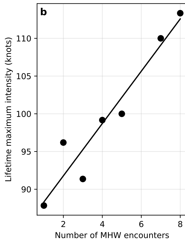
WP: MHW baseline 1992-2021
