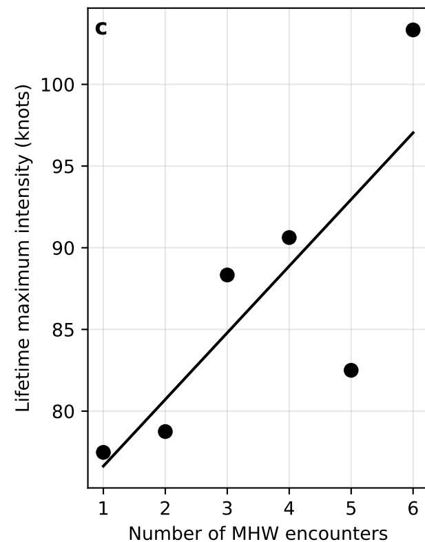
SH: MHW baseline 1992-2021
