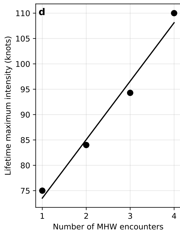
IO: MHW baseline 1992-2021
