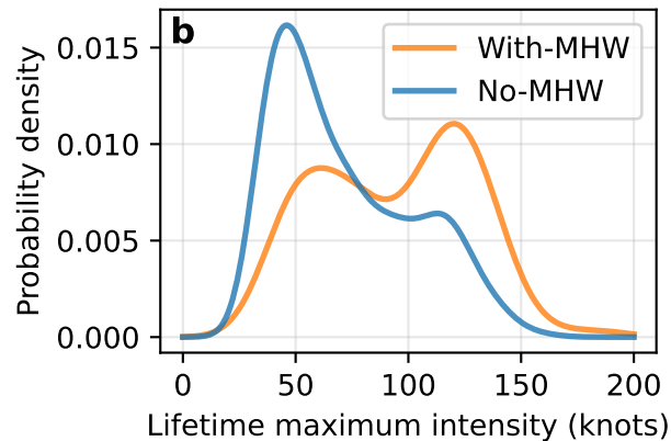
WP: MHW baseline 1992-2021
