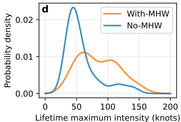
IO: MHW baseline 1992-2021
