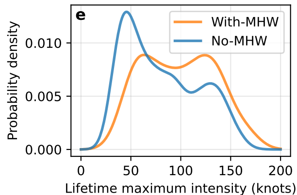
WP: MHW baseline 1992-2021
