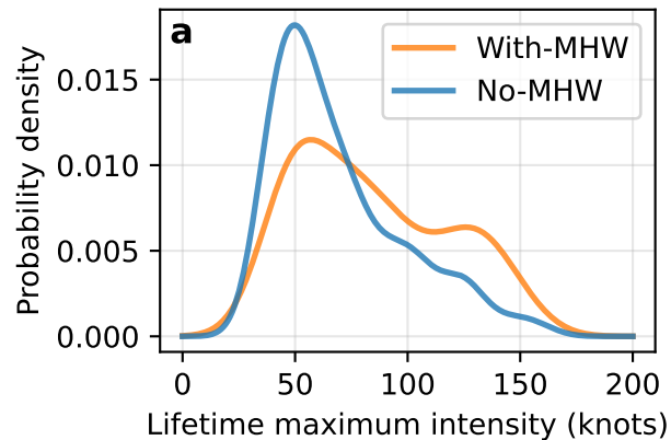
IO: MHW baseline 1992-2021
