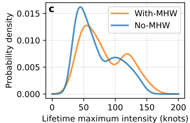
SH: MHW baseline 1992-2021
