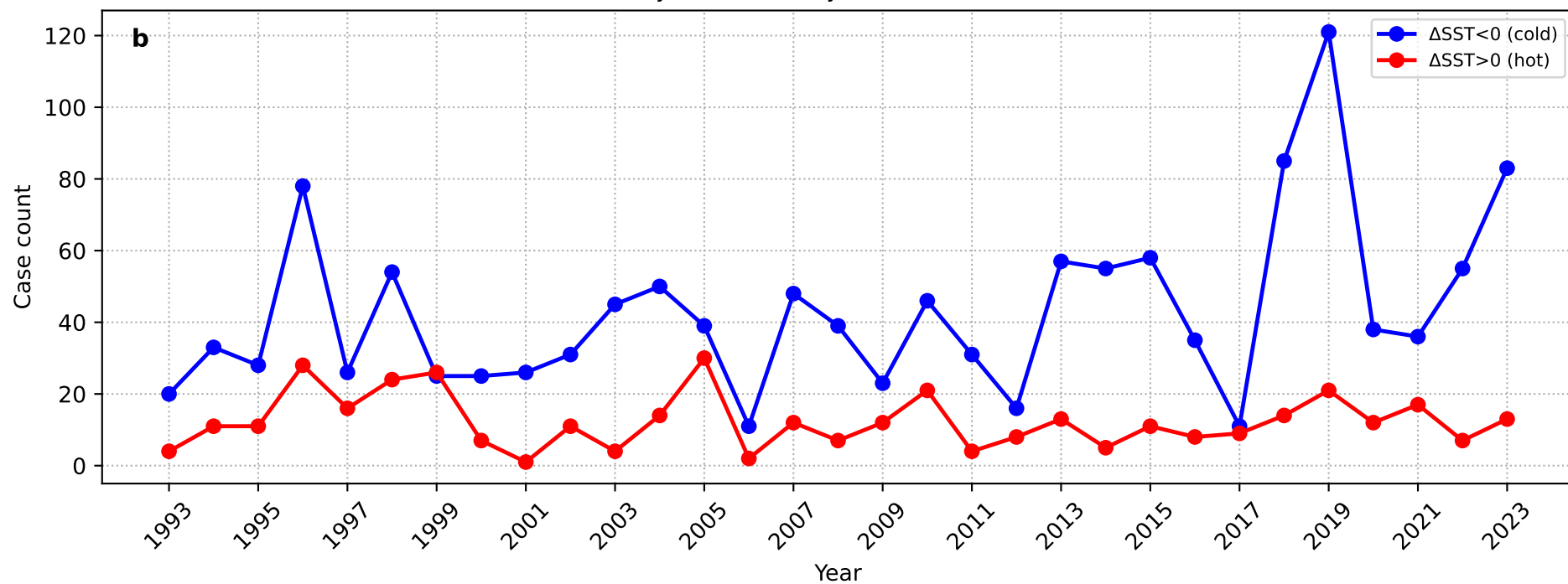
\Delta SST: Day 0 – mean(Day –10...–4) (IO + HYCOM)
