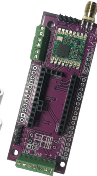
For SOLAR
