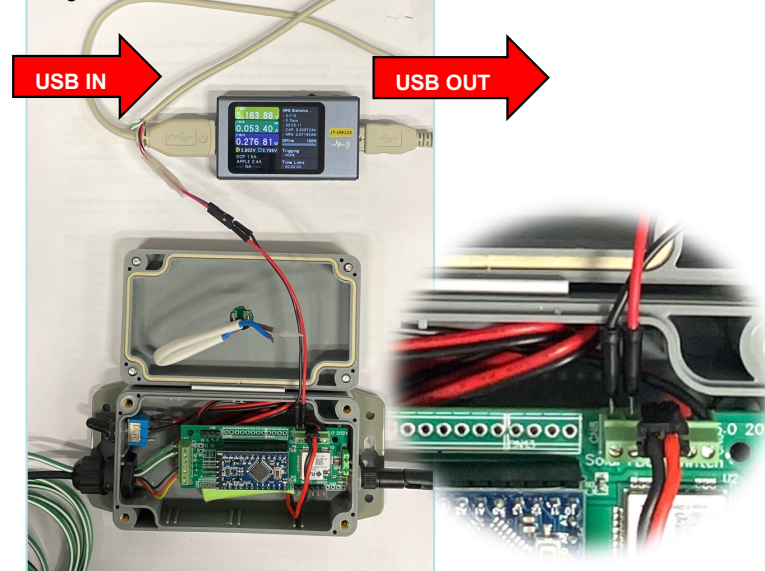
Image shown is the PCBA v5 from INTEL-IRRIS
