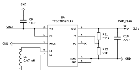
3.3V output buck-boost regulator
