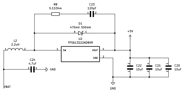
5V output boost regulator
