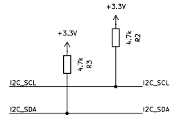
I2C interface pull up line
